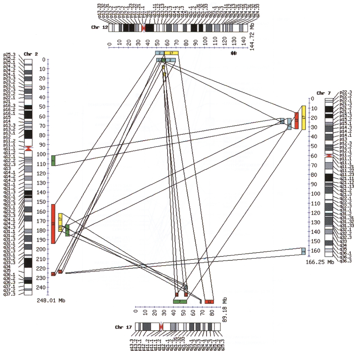
Figure 3. Blocks between Hox chromosomes. All detected paralogous blocks containing 6 or more duplicated genes between human chromosomes 2, 7, 12 and 17 are shown. Blocks can be viewed at wolfe.gen.ted.ie/dup .
