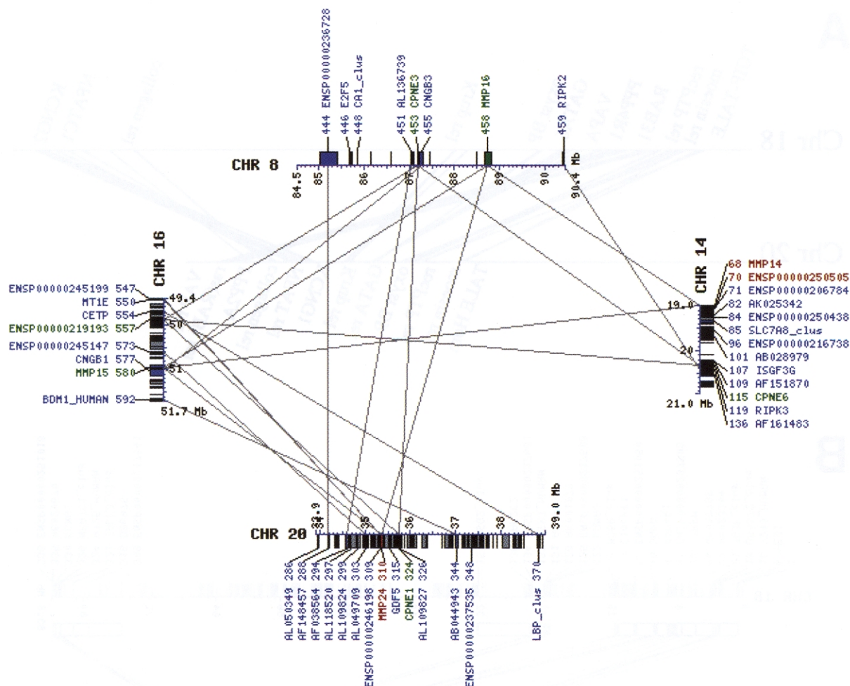
Figure 4. Blocks with copines and MMPs. The core areas of duplicated regions between human chromosomes 8, 14, 16 and 20 are shown. A copine (CPNE) and a matrix metalloproteinase (MMP) can be found in each of them in close vicinity (protein ENSP00000219193 on chromosome 16 is predicted to be a copine by the Ensembl automated annotation system). Linked genes are drawn and labelled in blue. Genes with links to two or three other blocks are highlighted in red and green, respectively. Intermediate genes are filled with grey.
