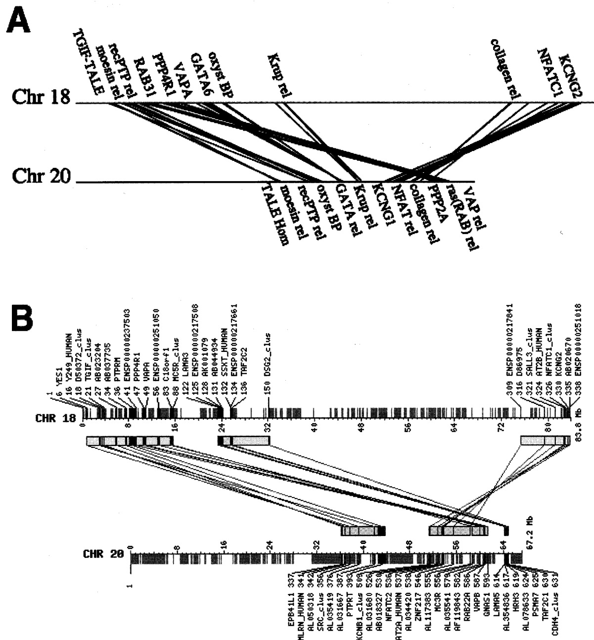
Figure 5. Paralogous regions between human chromosomes 18 and 20 defined by two different methods. Lines drawn between the chromosomes connect paralogues. (A) From Venter et al. (2001), showing labels for a selection of genes. (B) From our analyses with all duplicated genes labelled.
