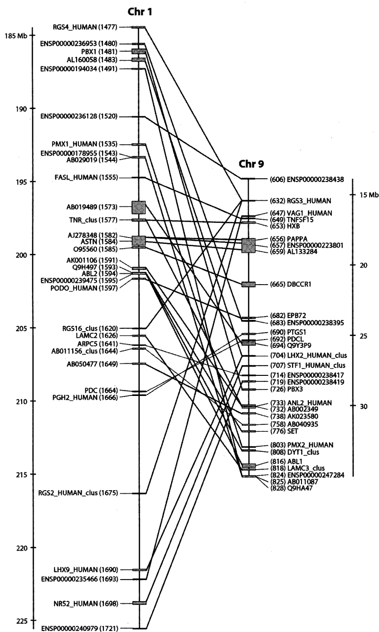
Figure 2. Paralogous block between human chromosomes 1 and 9. This is the largest paralogous block detected in the human genome including 29 duplicated genes. Blocks can be viewed at wolfe.gen.tcd.ie/dup .
