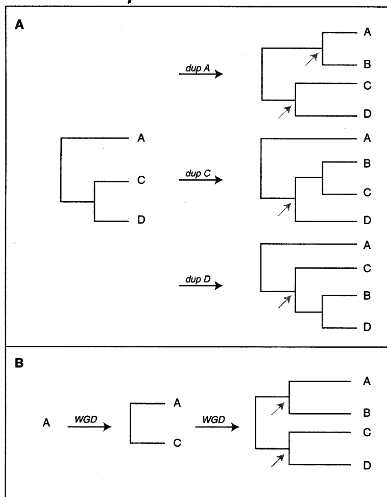
Figure 1. Alternative phylogenetic tree topologies of four-membered families resulting from sequential gene duplication or genome duplication. Grey arrows indicate the nodes that are critical to define the symmetry or asymmetry of the topology. (A) Phylogenetic tree topologies resulting from duplication of one member of a three-membered gene family. Three different trees result. The tree from the duplication of gene C and that from the duplication of gene D have asymmetric topologies. (B) Phylogenetic tree topologies resulting from two whole genome duplication (WGD) events. All genes are duplicated at each step, resulting in a symmetric tree topology.
